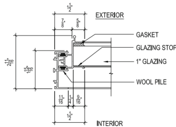
A CITIQUIET INTERIOR SLIDER JAMB DETAIL SCALE: 1" = 1"
