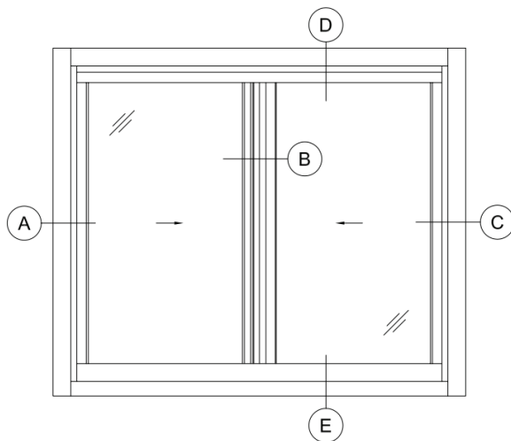
1 CITIQUIET INTERIOR SLIDER WINDOW EXTERIOR VIEW
