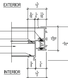
C CITIQUIET INTERIOR SLIDER JAMB DETAIL SCALE: 1" = 1"
