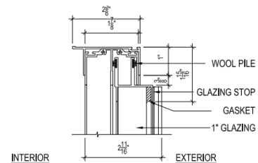
D CITIQUIET INTERIOR SLIDER HEADER DETAIL SCALE: 1" = 1"
