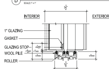
E CITIQUIET INTERIOR SLIDER SILL DETAIL SCALE: 1" = 1"
