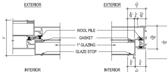
B CITIQUIET INTERIOR MEETING RAIL DETAIL SCALE: 1" = 1"
